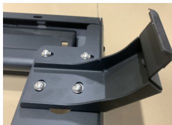
Inner support brackets fitted to the rack, and all 6 brackets installed.
